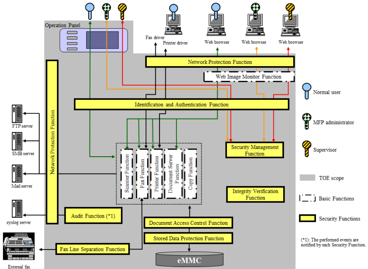
Figure 5-1 TOE Components
